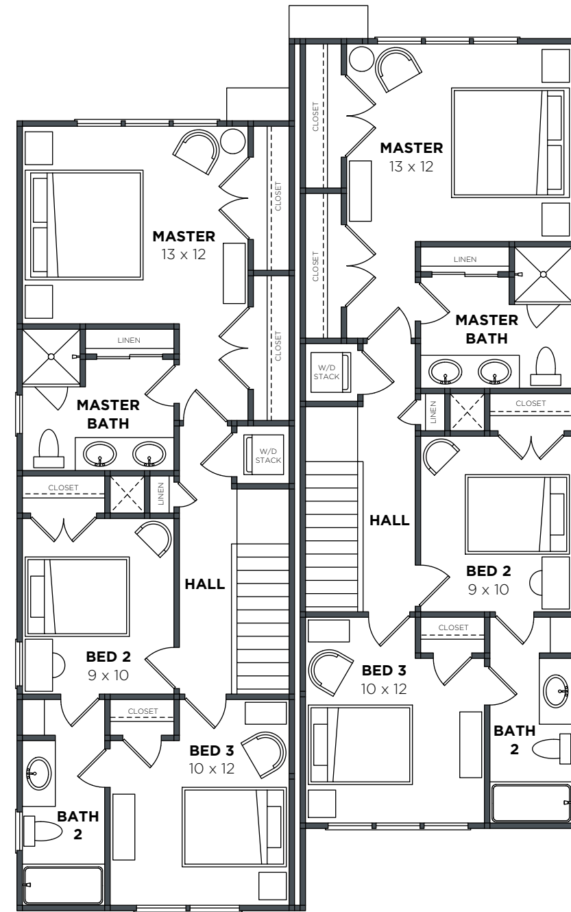
SECOND FLOOR
